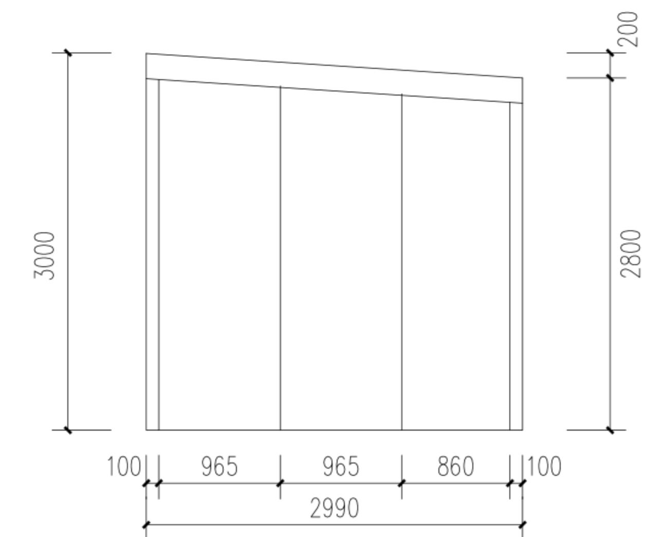
6 Right Elevation Scale: Approximate
