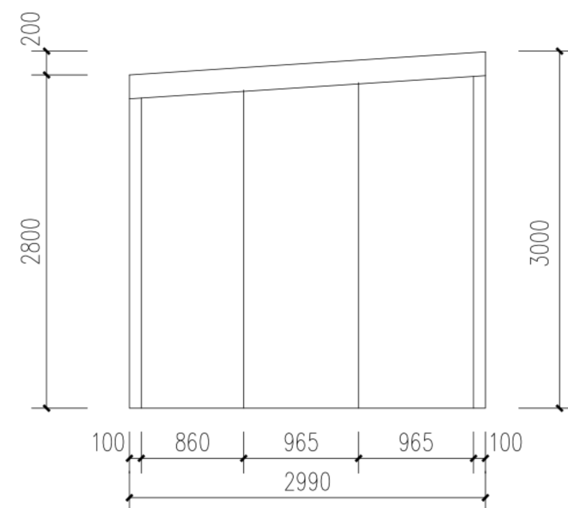
4 Left Elevation Scale: Approximate
