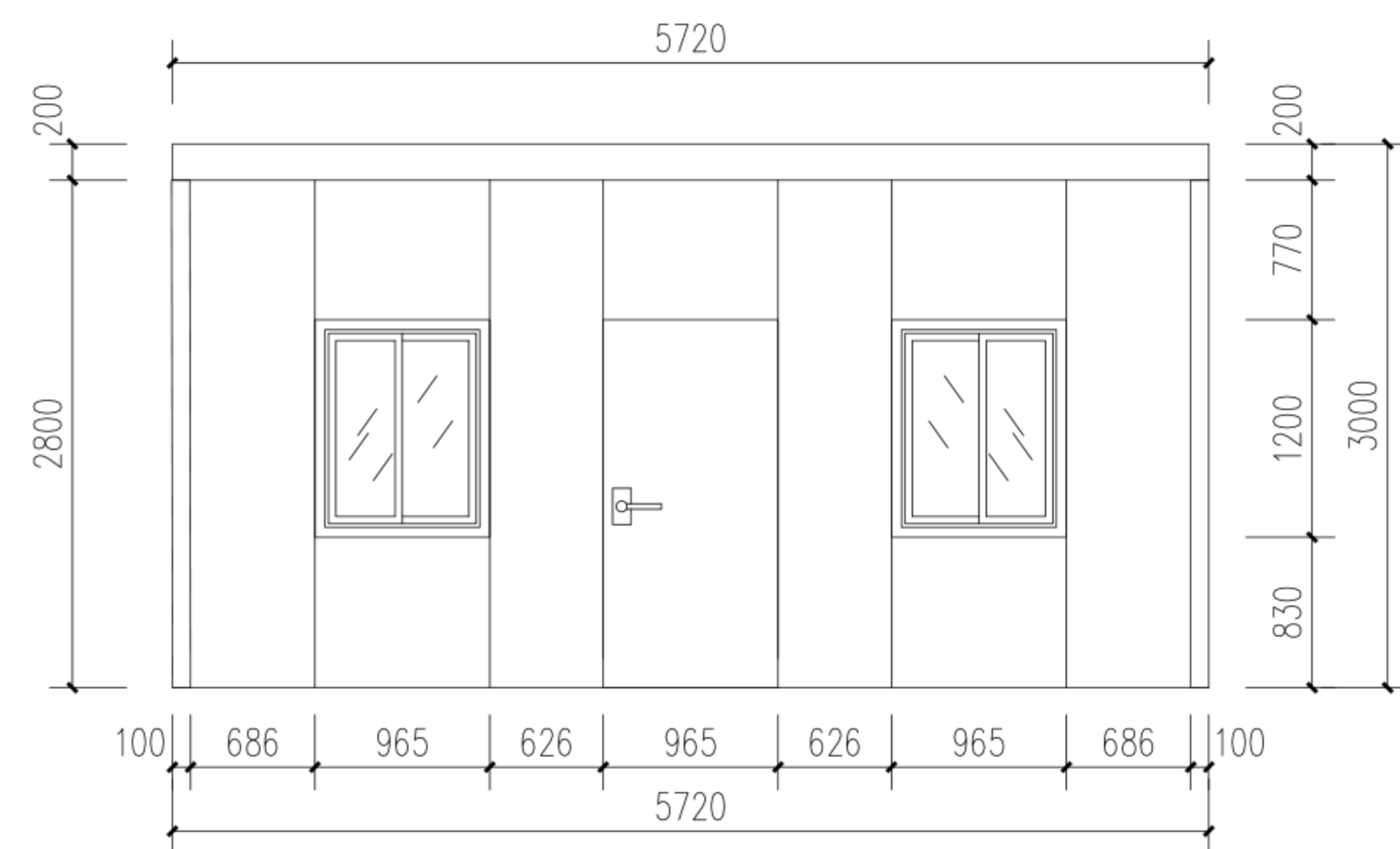
1 Front Elevation Scale: Approximate
