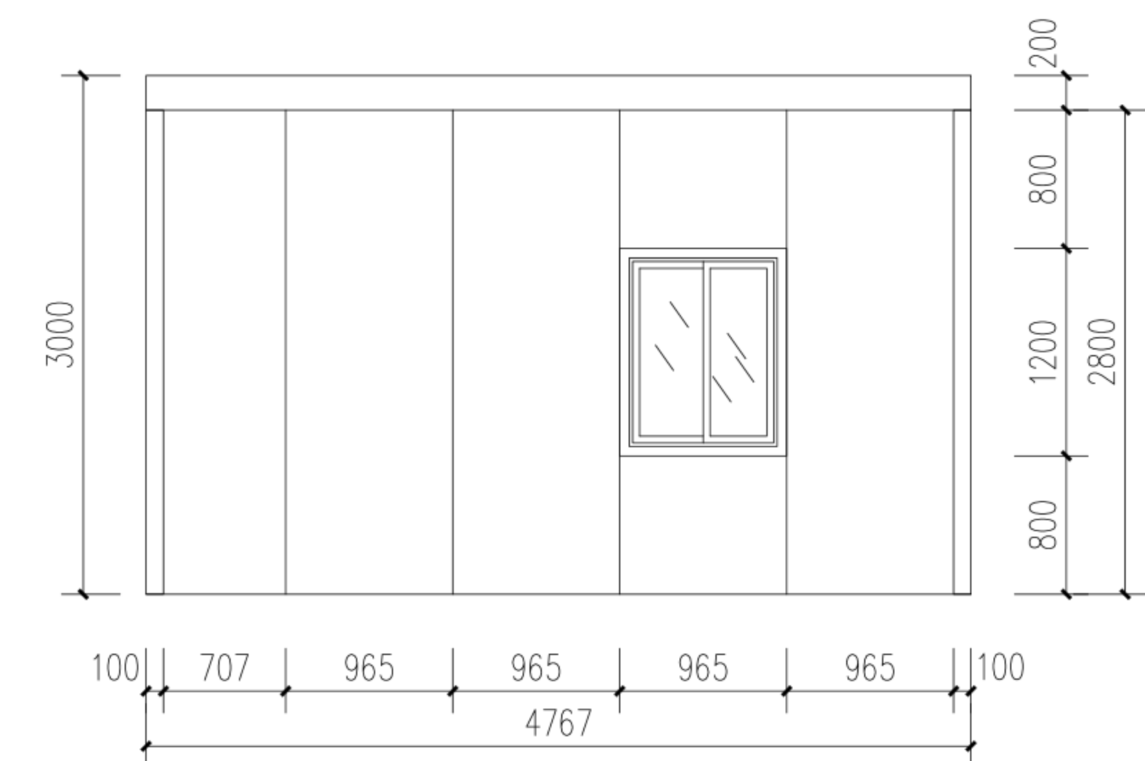
3 Rear Elevation Scale: Approximate
