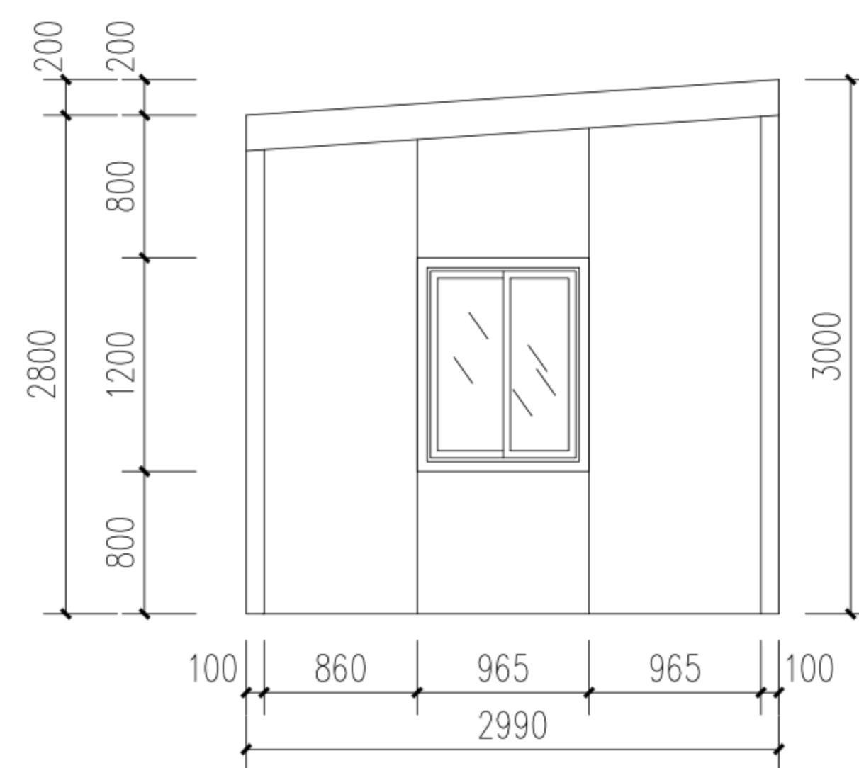
1 Front Elevation Scale: Approximate
