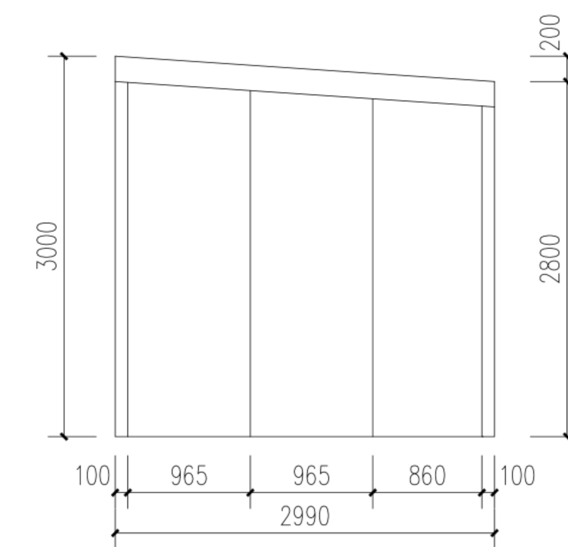
3 Rear Elevation Scale: Approximate
